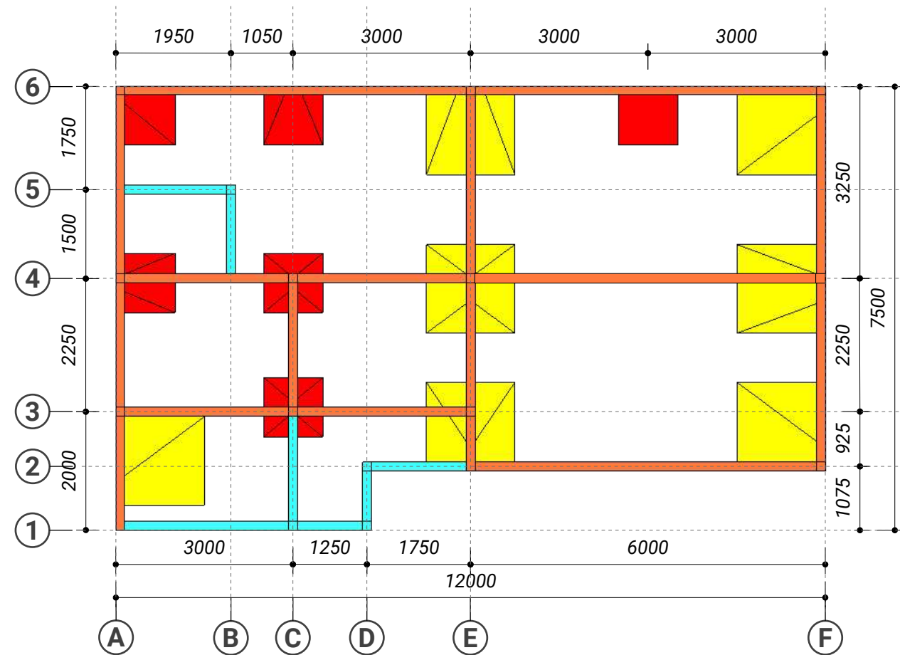
DENAH FOOTPLAT & SLOOF skala 1 : 100
