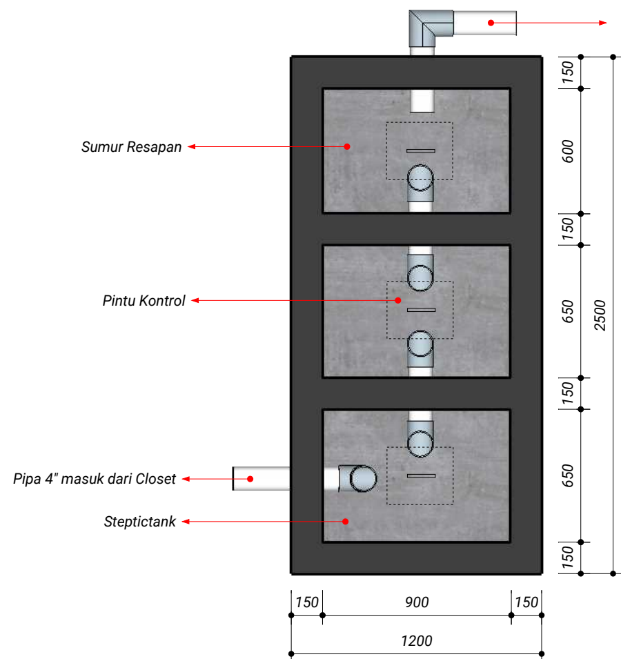
DENAH STEPTICTANK skala 1 : 50
