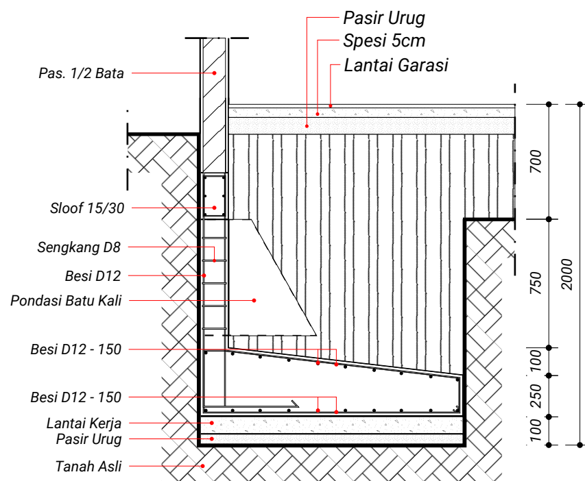
DETAIL FOOTPLAT 1 skala 1 : 20
