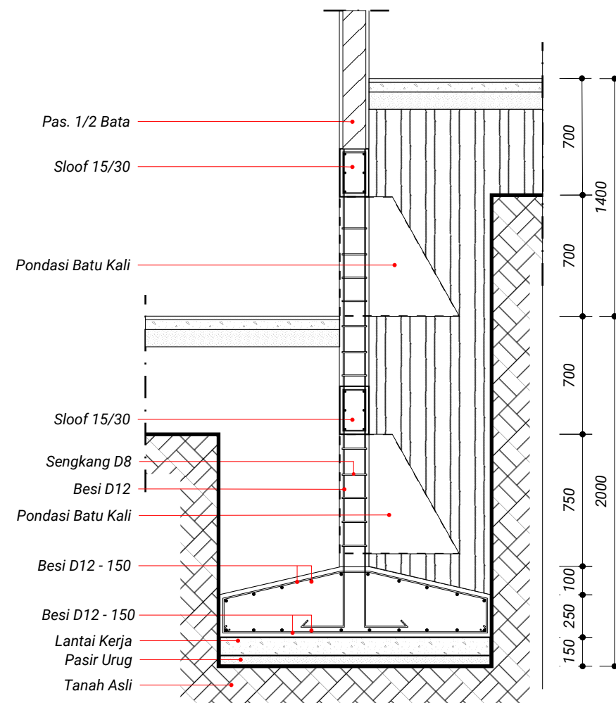
DETAIL FOOTPLAT 3 skala 1 : 20
