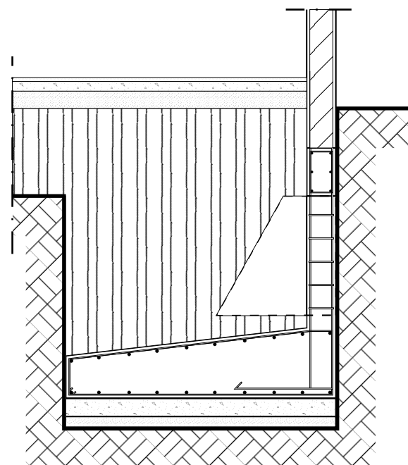
DETAIL FOOTPLAT 2 skala 1 : 20
