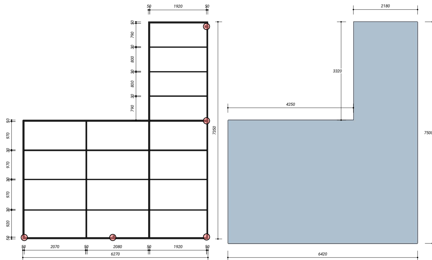
DENAH CANOPY skala 1 : 50
