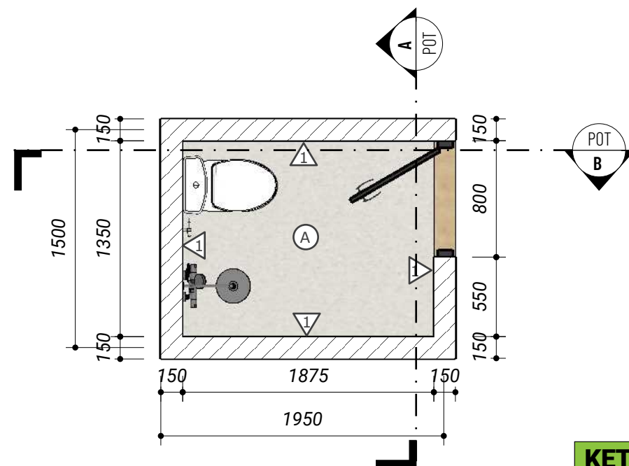
DENAH KAMAR MANDI 1 skala 1 : 50
