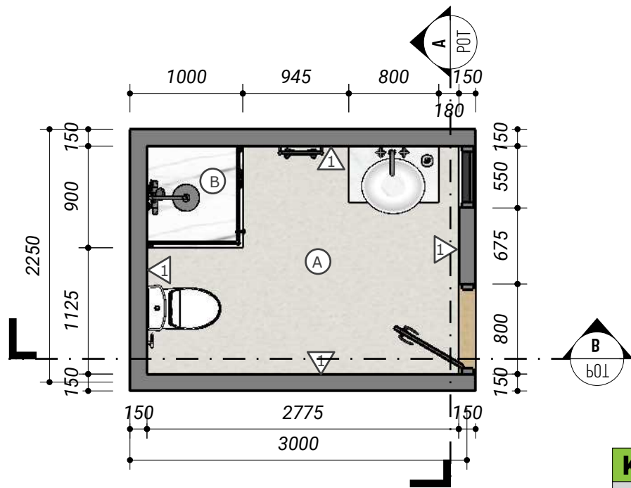
DENAH KAMAR MANDI 2
