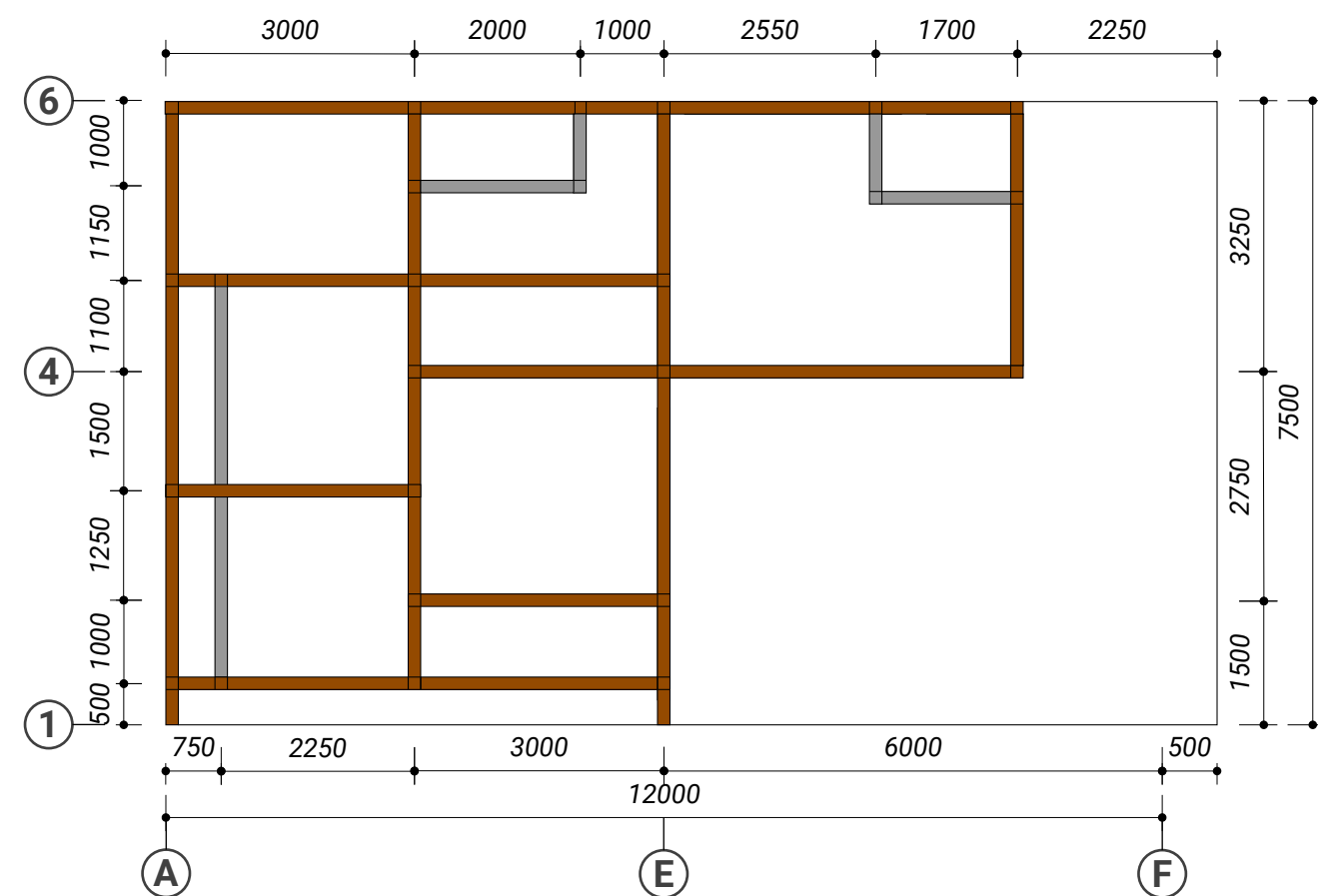
DENAH RING BALK skala 1 : 100
